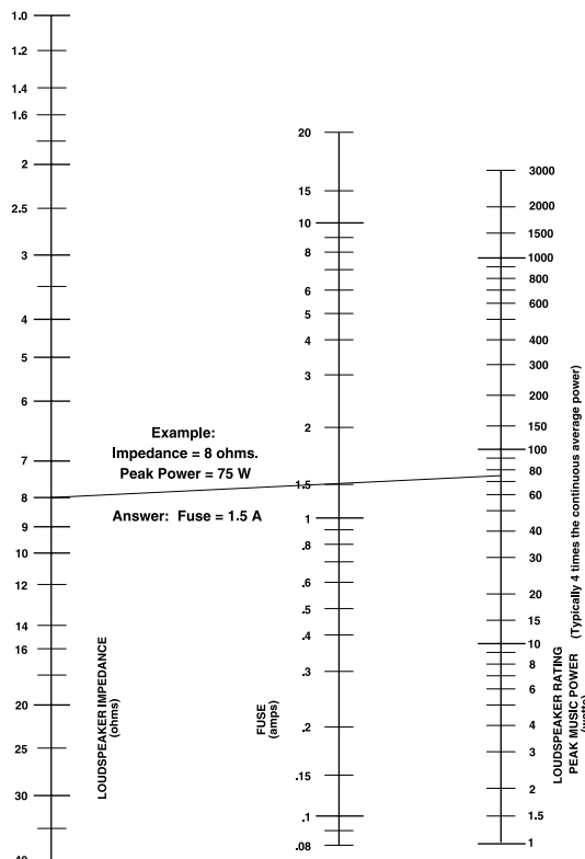
Figure 1.24 Loudspeaker Fuse Nomograph
